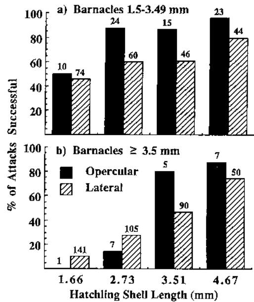
FIG. 8. Percent of attacks by hatchling Nucella emarginata that were successful at two different attack regions (opercular, lateral) as a function of hatchling and barnacle size (barnacles were pooled from all cages; attacks at both sites pooled). Numbers above each bar indicate sample sizes. Statistical analysis shown in Table 4e.
