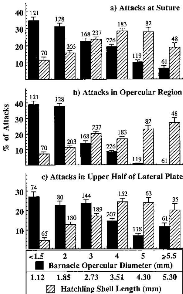
FIG. 5. Percent of attacks ( \bar{X} \pm \text{se} ) by hatchling Nucella emarginata at different locations on the skeleton of barnacles as a function of barnacle size and hatchling size: (a) attacks at sutures vs. attacks not at sutures of skeletal plates (data for opercular and lateral region pooled), (b) attacks in opercular vs. lateral region (data for attacks at sutures and plate margins pooled), (c) attacks in upper vs. lower half of lateral plates (data for lateral region only; attacks at sutures and plate margins pooled). Number above each bar indicates the size of the sample for which the percent was computed. Attacks as a function of barnacle opercular diameter (■) were pooled across all sizes of hatchlings. Attacks as a function of hatchling shell length (▨) were pooled across all sizes of barnacles. Opercular diameter class marks as in Fig. 1, hatchling shell lengths are class marks. Statistical analyses shown in Table 4a and 4b.
