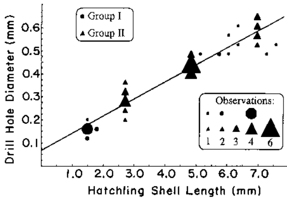
FIG. 3. Diameter of drill hole made by hatching Nucella emarginata as a function of hatching shell length. See Table 3 for regression equation and statistical analysis, and Results: Estimating Hatching Size From Drill Hole Diameter for a description of groups I and II.
