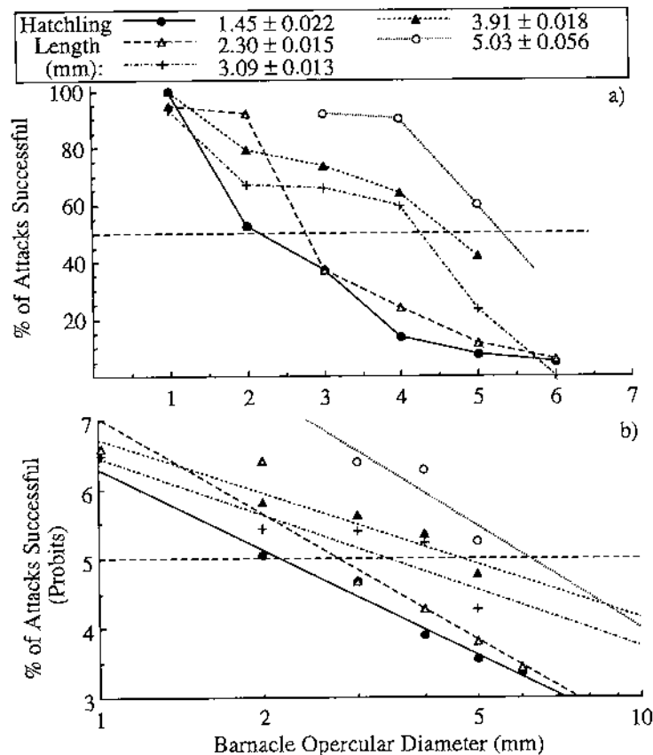
FIG. 9. Percent of attacks by hatchling Nucella emarginata that were successful, as a function of barnacle size, for each of five size categories of hatchlings (mean \pm SE): (a) raw percentages, (b) probit-transformed percentages from Table IX of Fisher and Yates (1943) with least squares regression lines. Total sample sizes for each hatchling size category were: 181, 194, 236, 136, and 76 for the smallest-to-largest size categories, respectively.
