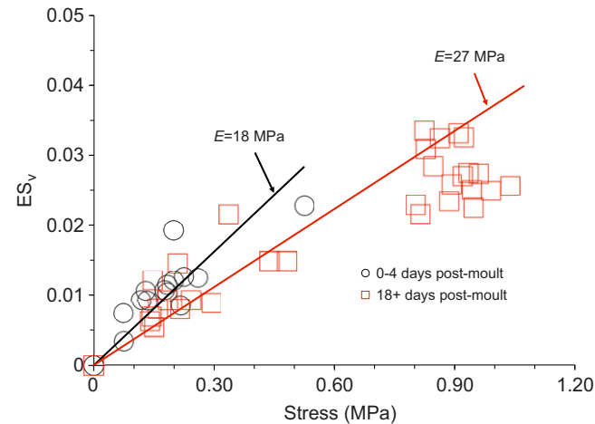
Fig. 3. Viscoelastic component of engineering strain ( ES_v ), for unfed ticks, as a function of applied stress to a maximum of 1.2 MPa. Data are from individual creep tests. Young's modulus ( E ) is calculated from the slope through the intercept. For ticks 0–4 days post-moult, y=0.0541x , and for ticks more than 18 days post-moult, y=0.0372x .
